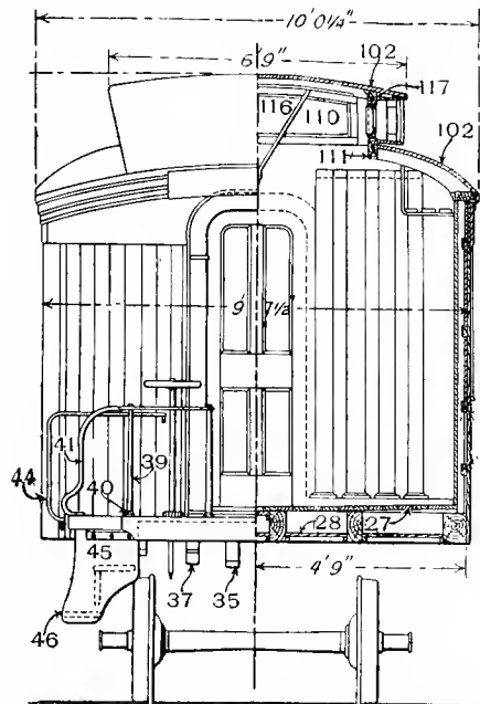
Fig. 511. End Elevation and Cross Section.
